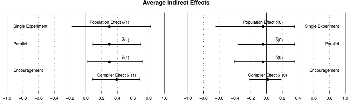
Figure 2: Identification Power of Alternative Experimental Designs. The graphs show the sharp bounds on the average indirect effects for the treatment (left panel) and control (right panel) conditions calculated on the basis of the hypothetical population distribution we generated. In each panel, the solid circles represent the true values of \bar{\delta}(t) (top three) and \bar{\delta}^*(t) (bottom). The horizontal bars indicate the sharp bounds under (from top to bottom) the single experiment design, parallel design, and parallel encouragement design. The graphs show improved identification powers of the new designs compared to the traditional single experiment design.
