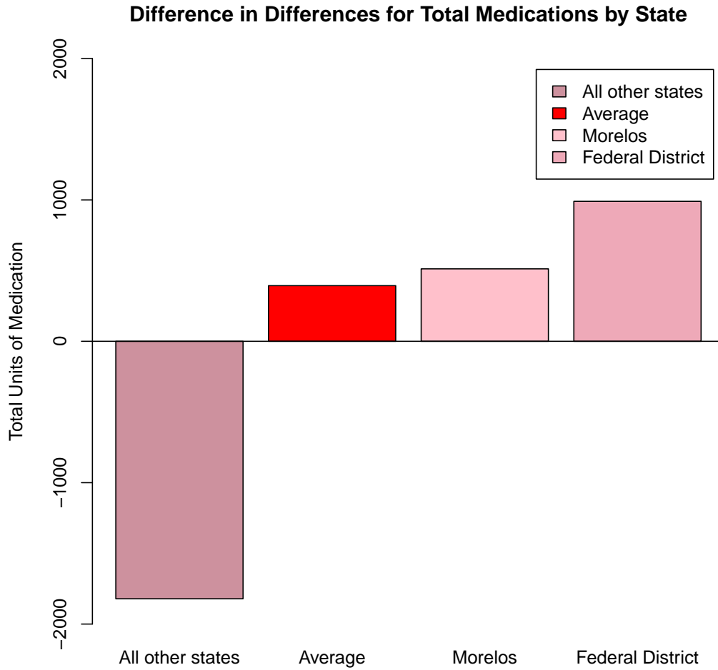
Figure 3: DID States
