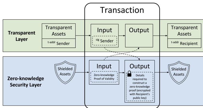
Figure 2.1: Depiction of a Z-cash transaction utilizing Zero-Knowledge proofs from [54]
