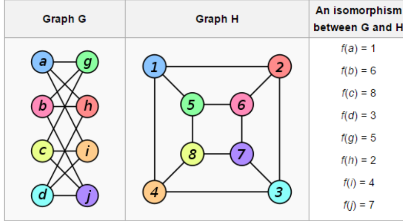
Figure 3.1: Demonstration of isomorphism between two undirected graphs G and H , from [25]
