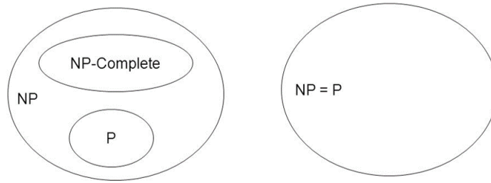
Figure 4.1: Left: If P \neq NP ; Right: If P = NP
