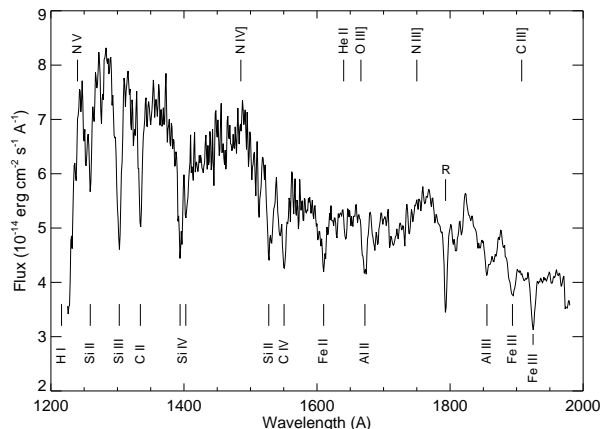
FIG. 1.—Reference SWP spectrum of stars 2 and 3 is the exposure-weighted sum of SWP 30592, 30637, and 30743. The principal stellar and interstellar absorption features are identified below the spectrum. The position of the six UV emission lines are marked above the spectrum. A prominent camera reseau is indicated by “R.”
