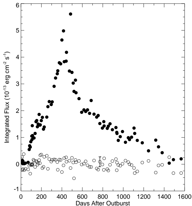
FIG. 7.—N v \lambda 1240 light curve (filled circles) and continuum residual, \delta F_c (eq. [1]), near the line are shown as a function of time. \delta F_c is a measure of the accuracy and consistency of the continuum placement used to compute the flux in the line (see Fig. 4). The results shown for N v are representative of the six lines measured. The error bar ( \pm 1 \sigma = 1.82 \times 10^{-14} \text{ erg cm}^{-2} \text{ s}^{-1} ) is the measurement uncertainty for individual data points.
