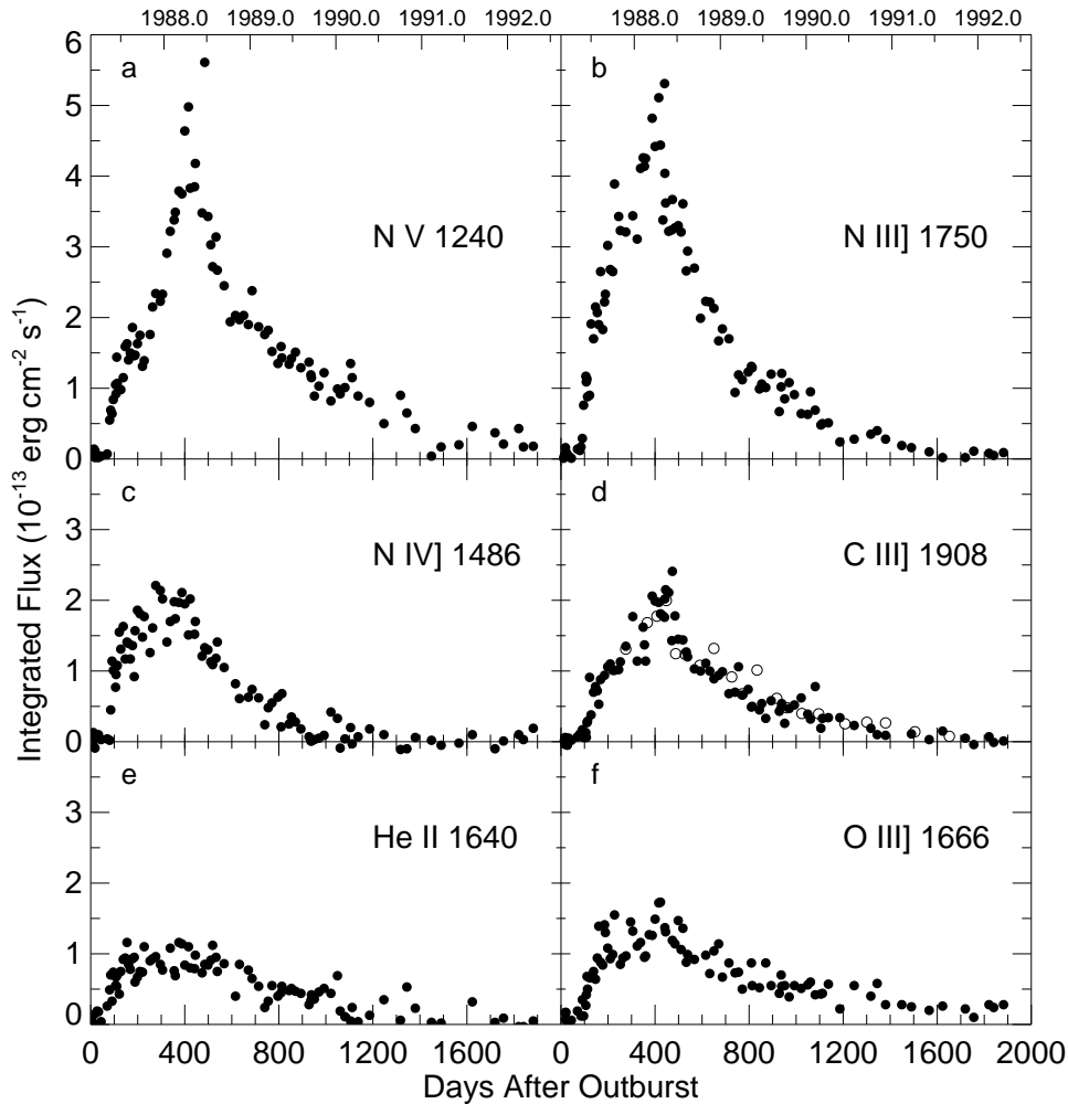
FIG. 6.—Light curves spanning day 11 to 1882 for the six UV emission lines in SN 1987A. The open circles in (d) are the combined C III] \lambda 1906.68 and \lambda 1908.73 fluxes from the IUE high-dispersion spectra (Table 2).
