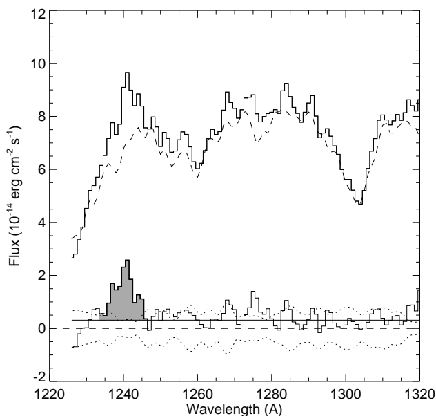
FIG. 4.—Continuum subtraction for N V in SWP 36801. The upper solid line is the observed SN 1987A spectrum. The upper dashed line is the reference spectrum of stars 2 and 3 from 1987 March (see Fig. 1). The difference spectrum ( SN-stars ) is shown by the solid line at the bottom of the figure on the same flux scale. The solid horizontal line is the continuum level established for this N V flux measurement ( shaded area ). The dashed horizontal line marks the zero flux level. The N V emission feature is more easily distinguished in the difference spectrum. The dotted lines above and below the difference spectrum are the \pm 1 \sigma residuals for the reference spectrum. Cross-correlation techniques were used to register the SN 1987A and star 2 and 3 spectra; a +93 \text{ km s}^{-1} correction was applied to the reference spectrum in this example.
