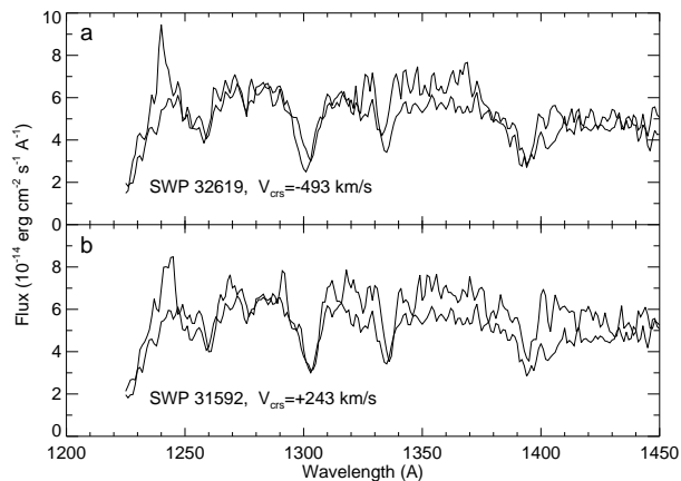
FIG. 2.—Two SWP spectra of SN 1987A ( thicker lines ) illustrating the effect of the changing orientation of stars 2 and 3 with respect to the dispersion axis. The SWLA position angles for the two spectra differ by 156^\circ . The reference spectrum of stars 2 and 3 (see Fig. 1) is shown by the thinner line.
