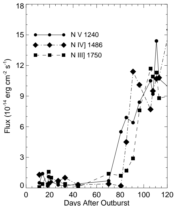
FIG. 9.—Comparison of the three nitrogen emission-line light curves before day 120. The sudden onset of the lines also indicates a progression from higher to lower ionization potential.
