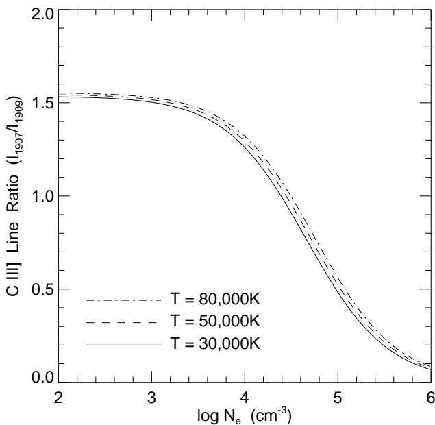
FIG. 13.—Calculated C III] line ratios ( I_{1907}/I_{1909} ) as a function of n_e for a six-level C III atom are shown for electron temperatures of 30,000 K, 50,000 K, and 80,000 K. The atomic data are from several sources: A -values for C III from Nussbaumer & Storey (1978), Allard et al. (1990), and Fleming et al. (1994), energy levels are those of Mendoza & Zeippen (1983) and Aggarwal et al. (1986), and collision strengths from Seaton (1987) and Keenan et al. (1992).
