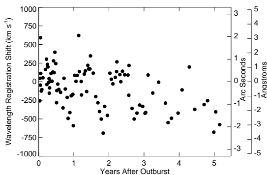
FIG. 3.—Wavelength (velocity) registration shift for the SN 1987A SWP database, as determined by cross-correlation with the star 2 and 3 reference spectrum, shown as a function of time. The right-hand axes show the corresponding spatial and wavelength scales. The scatter at the level of \pm 125 \text{km s}^{-1} is a measure of the accuracy with which the supernova is centered in the aperture. The 1 year cycle of aperture rotation on the sky produces the long-term variation.
