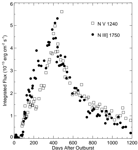
FIG. 8.—Comparison of the N iii] and N v light curves near maximum. The large deficiency of N v relative to N iii] before maximum is believed to be the result of resonant scattering by \text{N}^{+4} ions in the highly ionized gas close to the ring along the line of sight to the supernova.
