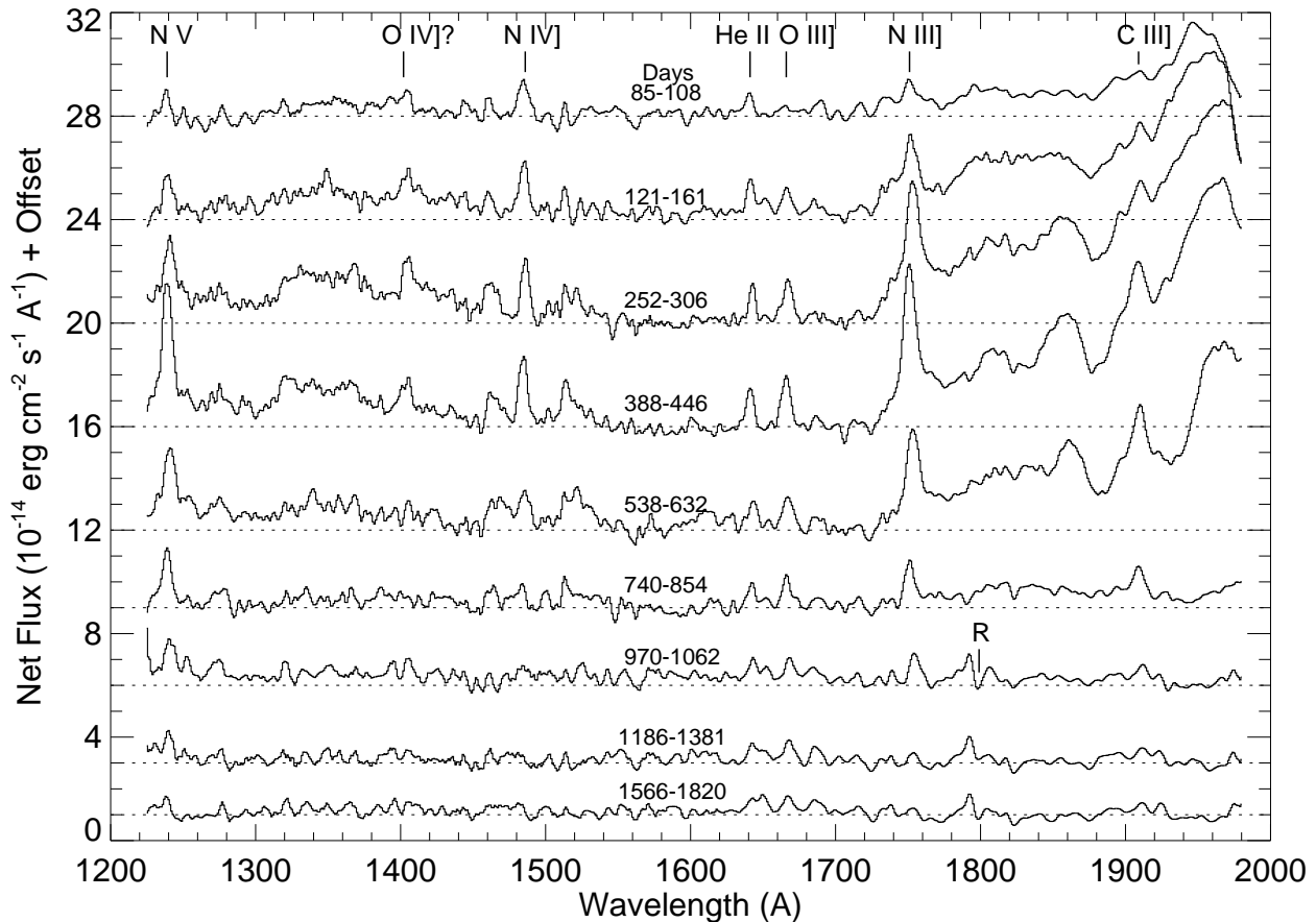
FIG. 5.—Mean SWP spectrum of SN 1987A (minus stars 2 and 3) is shown for nine time intervals spanning the first 1820 days of the outburst. Each mean spectrum is the average of five exposures over the indicated time interval. They are plotted on the same flux scale and are offset for clarity. The dashed horizontal lines mark the zero level for each spectrum. The six emission lines measured are marked at the top of the figure, as is the possible identification of O iv] multiplet UV 0.01.
