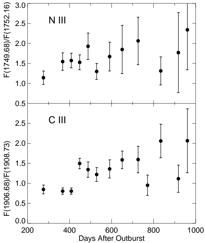
FIG. 12.—Evolution of the N III] \lambda 1749/\lambda 1752 and C III] \lambda 1907/\lambda 1909 line ratios between days 275 and 1000.
