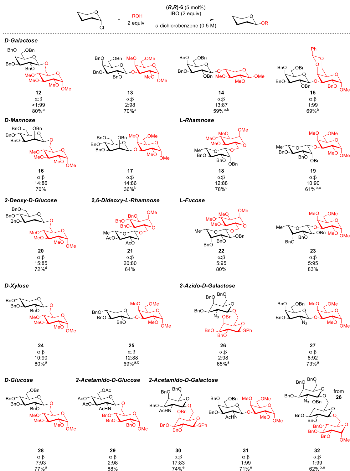
Fig. 3. Substrate Scope. Isolated yields are reported. Diastereomeric ratios were determined by NMR or HPLC analysis of crude material. * Reaction run at 40 °C. † Reaction run with 10 mol% catalyst. ‡ Reaction run at 0 °C with (S,S)-6. § Reaction run in toluene (0.1 M) at –40 °C. || Reaction run in dichloromethane.
