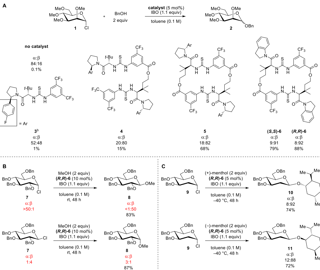
Fig. 2. Evaluation of reaction components. (A) Catalyst optimization. (B) Effect of glycosyl chloride configuration at the anomeric center. (C) Effect of nucleophile chirality.
