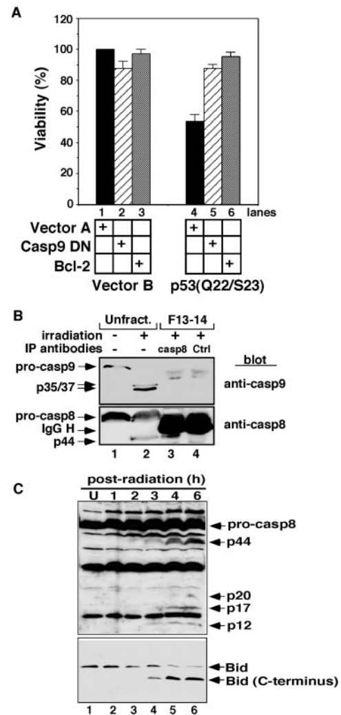
FIG. 5. Requirement for caspase-9 in transcription-independent apoptosis triggered by p53. A, Saos2 cells were cotransfected with pRSV-LacZ and expression vectors coding for either p53(Gln 22 /Ser 23 ), caspase-9 DN, or Bcl-2, as indicated. pcDNA3 (vector A) and pRc/CMV (vector B) were used as controls. 30 h after transfection, the cells were fixed and stained with X-gal. Viable blue cells, determined by morphology, were counted from 20 randomly selected fields (200X). Data were normalized to the vector control (defined as 100% survival) and are displayed as mean \pm S.E. from three experiments done in triplicate. B, extracts prepared from transformed p53 +/+ MEFs at 4 h following irradiation were fractionated by size exclusion chromatography using a Superose-6 HR column. Fractions 13–14 (F13–14), which contain the p44-processed form of caspase-8, were pooled and immunoprecipitated with either a rat antiserum against caspase-8 (lane 3) or a control rat serum (lane 4). The immunoprecipitates were analyzed by immunoblotting for the presence of caspase-9 (top panel) and caspase-8 (bottom panel). Unfractionated p53 +/+ extracts (unirradiated, lane 1; 4 h after irradiation, lane 2) were used as controls. The positions of procaspases and their processed forms are indicated. C, extracts were prepared from untreated (U) or irradiated, transformed p53 +/+ MEFs at the indicated time points (hours) after \gamma -irradiation. The proteins were separated by a 12.5% SDS-polyacrylamide gel and transferred to a nitrocellulose membrane. The membrane was then sequentially probed with antibodies against caspase-8 and the C terminus of Bid. Procaspase-8, its cleavage products (p44, p20, p17, and p12), and the C-terminal fragment of Bid are indicated.
