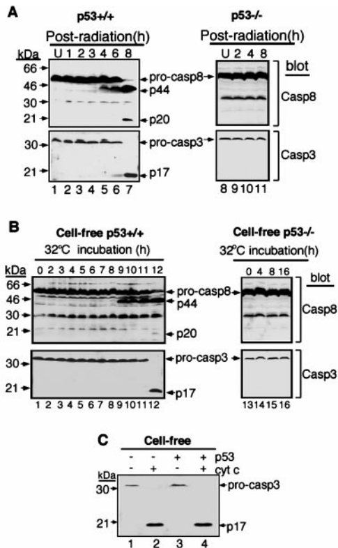
FIG. 1. Caspase-8 is activated early in p53-mediated apoptosis. A, caspase activation in transformed MEFs (p53 +/+ or p53 -/- ) following 10-gray irradiation. Extracts were prepared from untreated (U) or irradiated cells at the indicated time points (hours) after \gamma -irradiation. Activation of caspases was examined by immunoblotting with antibodies against individual caspases. The characteristic cleavage products of caspase-8 (p44 and p20) and caspase-3 (p17) are indicated. B, caspase activation in S100 cell-free extracts. Extracts were prepared from E1A/Ras-transformed MEFs (p53 +/+ or p53 -/- ) at 1 h after 10-gray irradiation and incubated at 32 °C for the indicated times, followed by immunoblot analyses for caspase activation. C, activation of caspase-3 in cell-free extracts by cytochrome c (cyt c ). Extracts were prepared from transformed MEFs (p53 +/+ or p53 -/- ) and incubated at 32 °C for 1 h in the absence or presence of cytochrome c (200 ng), followed by immunoblot analyses for caspase-3 activation.
