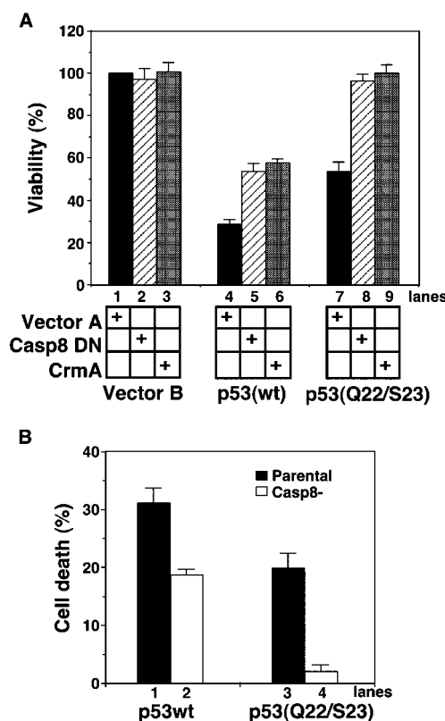
FIG. 3. Caspase-8 is required for transcription-independent apoptosis induced by p53. A , Saos2 cells were cotransfected with pRSV-LacZ and expression vectors coding for either wild-type p53, p53(Gln 22 /Ser 23 ), caspase-8 (C360S), or CrmA, as indicated. pcDNA3 (vector A) and pRe/CMV (vector B) were used as controls. 30 h after transfection, the cells were fixed and stained with X-gal. Viable blue cells, determined by morphology, were counted from 20 randomly selected fields (200X). Data were normalized to the vector control (defined as 100% survival) and are displayed as mean \pm S.E. from representative experiments done in triplicate. B , the parental and caspase-8-deficient mutant Jurkat cells were cotransfected with pEGFP and either pCMV-p53(wt) or pCMV-p53(Gln 22 /Ser 23 ). 24 h after transfection, apoptotic cells were quantitated by annexin V-based fluorometric assays. Data are mean \pm S.D. from four experiments.
