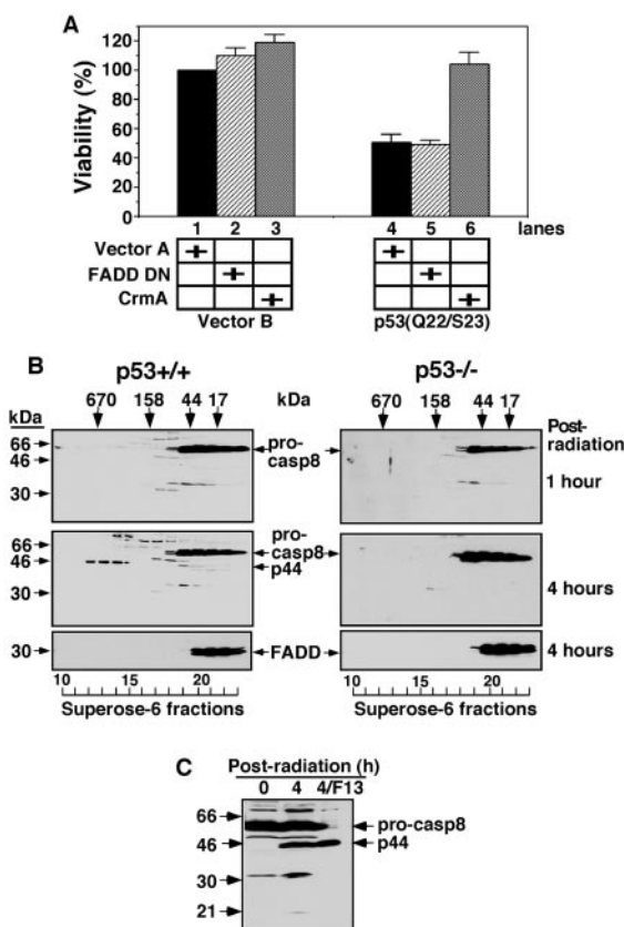
FIG. 4. FADD is not required for p53-dependent apoptosis. A , Saos2 cells were cotransfected with pRSV-LacZ and expression vectors coding for either p53(Gln 22 /Ser 23 ), FADD DN, or CrmA, as indicated. pcDNA3 (vector A) and pRe/CMV (vector B) were used as controls. 30 h after transfection, the cells were fixed and stained with X-gal. Viable blue cells, determined by morphology, were counted from 20 randomly selected fields (200X). Data were normalized to the vector control (defined as 100% survival) and are displayed as mean \pm S.E. from representative experiments done in triplicate. B , extracts prepared from transformed p53 +/+ or p53 -/- MEFs at indicated hours following irradiation were fractionated by size exclusion chromatography using a Superose-6 HR column. Aliquots (100 \mu l) of the indicated fractions were analyzed by immunoblotting for the presence of procaspase-8, its processed form (p44), and FADD. The elution positions of molecular weight markers are indicated. C , unfractionated p53 +/+ extracts (untreated or 4 h after irradiation) and fraction 13 of the p53 +/+ 4-h extracts (shown as U, 4, or 4/F13) were analyzed by immunoblotting with an antibody against caspase-8. Procaspase-8 and its processed p44 form are indicated and demonstrate that the caspase-8 species in fraction 13 co-migrates with p44.
