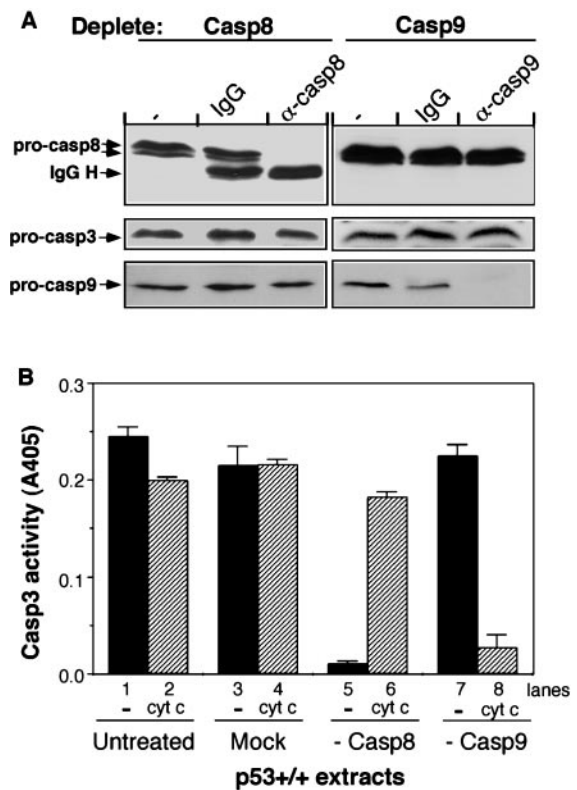
FIG. 2. Caspase-8 is required for caspase-3 activation in p53-dependent cell-free extracts. A, immunodepletion of caspase-8 or -9. Extracts were prepared from transformed p53 +/+ MEFs at 1 h after 10-gray irradiation. Caspase-8 or -9 was depleted from the extracts with a rat antiserum against mouse caspase-8 or rabbit polyclonal IgG against caspase-9. Control immunodepletion was performed with normal rat serum or rabbit IgG. The immunoblots were sequentially probed with antibodies against caspase-8, -3, and -9. The position of rat IgG heavy chain (IgG H) is indicated. B, colorimetric assays of caspase-3 activity. Extracts containing or lacking caspase-8 or -9 were incubated at 32 °C either for 12 h in the absence of cytochrome c or for 1 h in the presence of cytochrome c (200 ng). The caspase-3 substrate DEVD-pNA was then added for 30 min at 32 °C. Caspase-3 activity was determined by measuring the cleavage of DEVD-pNA. Data are mean \pm S.D. from three independent experiments. p53-dependent apoptosis (black bars) was ablated by depletion of caspase-8 but was intact following depletion of caspase-9. In contrast, cytochrome c -mediated activation was ablated by depletion of caspase-9 but was intact following depletion of caspase-8.
