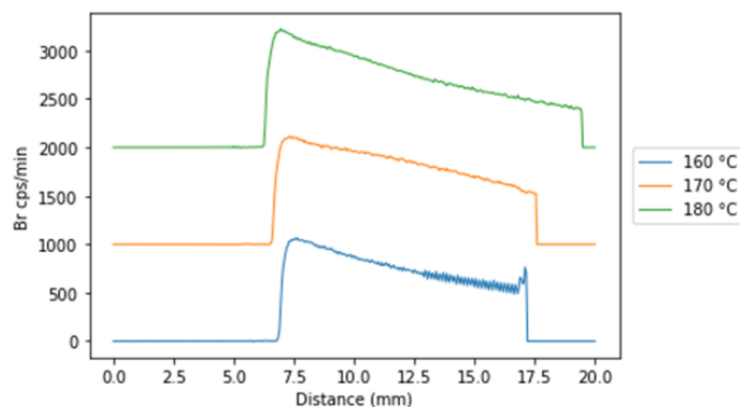
Figure 4-26: Br EDS intensity signals from a \text{SnBr}_2 sample deposited with 0.4 sccm HBr and 0.05 sccm \text{Sn}(\text{acac})_2 at temperatures 160, 170, and 180 °C.
