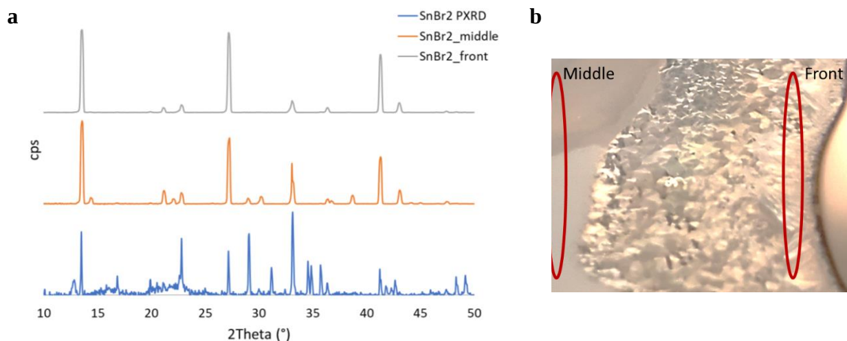
Figure 4-3: a) XRD of \text{SnBr}_2 film deposited at 120\text{ }^\circ\text{C} with 0.4\text{ sccm} \text{HBr} and ca. 0.05\text{ sccm} \text{Sn}(\text{acac})_2 for 15\text{ min} . The “front” and “middle” of the film can be seen in the example image in b), where the front is the area closest to the gas injector inlet manifold and the middle is further away.
