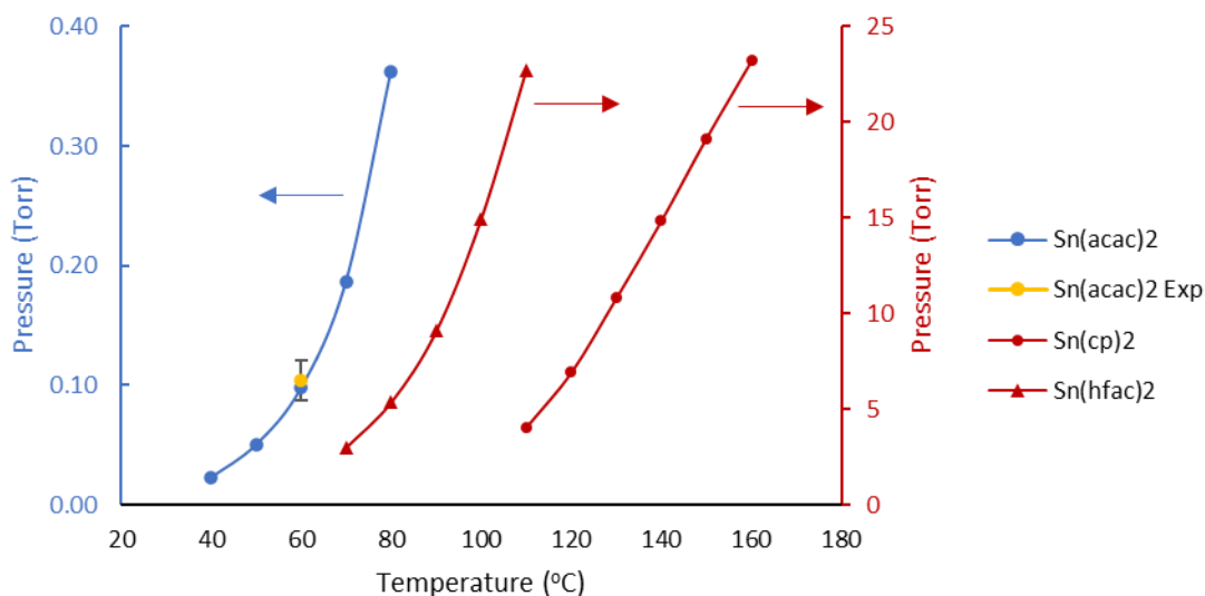
Figure 2-7: Vapor pressure estimates of \text{Sn}(\text{acac})_2 , \text{Sn}(\text{hfac})_2 , and \text{Sn}(\text{cp})_2 from TGA measurements. The TGA vapor pressure estimates were derived assuming a Langmuir evaporation model using benzyl alcohol reference TGA data together with their respective vapor pressures. 9-12 The experimental value for the vapor pressure of \text{Sn}(\text{acac})_2 at 60 °C was estimated from bubbling 250 sccm of \text{N}_2 through a \text{Sn}(\text{acac})_2 bubbler at 60 °C for 120 min and collecting the vapor in a liquid nitrogen cold trap. The \text{Sn}(\text{acac})_2 was transferred and weighed inside a glovebox. The error estimates include \pm 10 mg.
