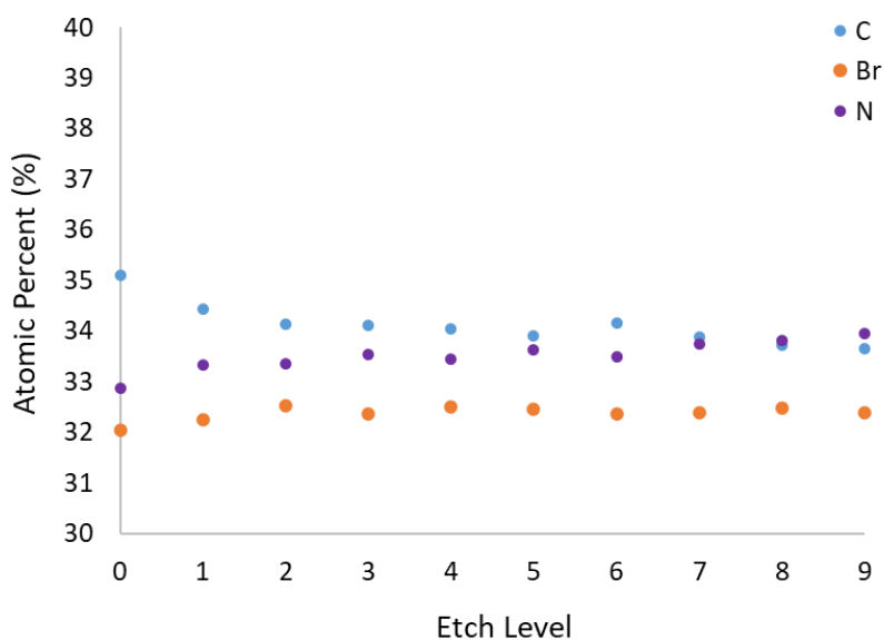
Figure 4-5: XPS atomic percent of a representative MABr film deposited at 120 °C for 5 min with 0.45 sccm of HBr and 0.25 sccm of MA.
