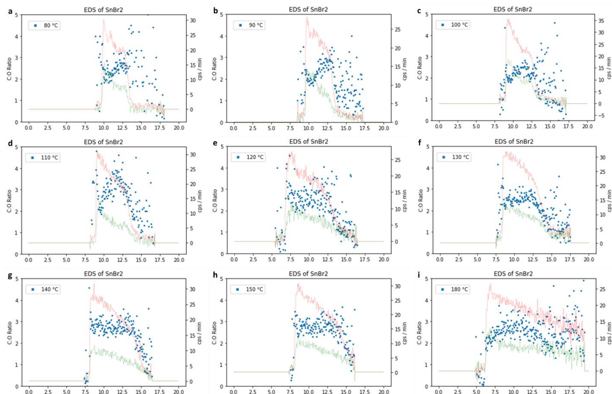
Figure 4-28: (a-i) C and O EDS signals on the right axis and their ratio on the left axis. The data was collected from \text{SnBr}_2 depositions made with 0.4 sccm of \text{HBr} and 0.05 sccm of \text{Sn}(\text{acac})_2 between temperatures of 80—180 °C. Notably, the ratio of C:O is near 2.5, the ratio of C to O in acetylacetone and the acetylacetonate anion ( \text{Acac}^- ). The abscissa is the distance, measured in millimeters, from the center of the reactor.
