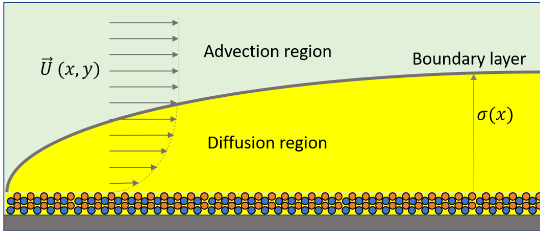
Figure 2-2: Boundary layer
