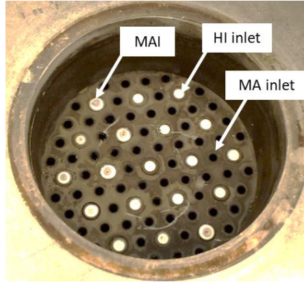
Figure 3-1: Reaction of methylamine (MA) and HI to make MAI that clogged the HI inlets. This demonstrated a need to use a nitrogen gas curtain to initially separate the precursors.
