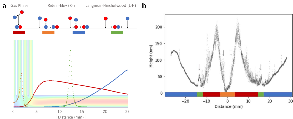
Figure 4-9: (a) The 4 reaction models considered show strong spatial dependencies. Four generic simulations for the deposition of MABr, one for each reaction model, are overlayed on half of the corresponding velocity map of the Gen 1 reactor. (b) MABr profilometry data for a deposition at 60 °C with 0.13 sccm of HBr and MA suggests multiple reaction mechanisms determined the film thickness. The color bar corresponds to the different reaction mechanisms suggested in (a). The arrows indicate possible contributions from gas-surface reactions to the overall film deposition.
