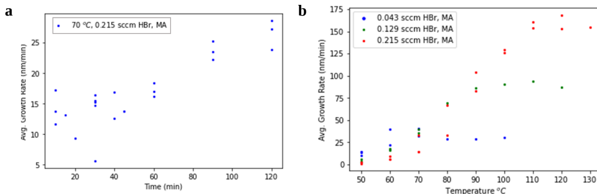
Figure 4-16: The average growth rate (nm/min) was calculated by normalizing the average profilometry height across 50 mm of the sample by the duration of the deposition. (a) Experiments that varied the deposition duration while keeping the temperature fixed at 70 °C suggested the average growth rate was constant up to 60 min and then increased beyond 60 min of deposition. (b) When the temperature was varied and the deposition duration was fixed at 30 min, the average growth rate appeared to linearly increase until a saturation plateau was reached.
