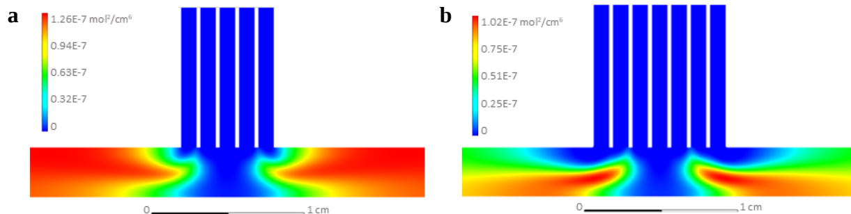
Figure 3-8: The extra flanking N 2 curtains (b) act to suppress the product of the concentrations of HI and MA over the design with only 2 N 2 curtains (a). The legend shows the product of the concentrations of HI and MA. The input conditions were 250 sccm for each channel with 0.1% MA and 0.15% HI in N 2 . The results for HI were expected to carry over to HBr given that they are very similar and have a similar diffusion coefficient.
