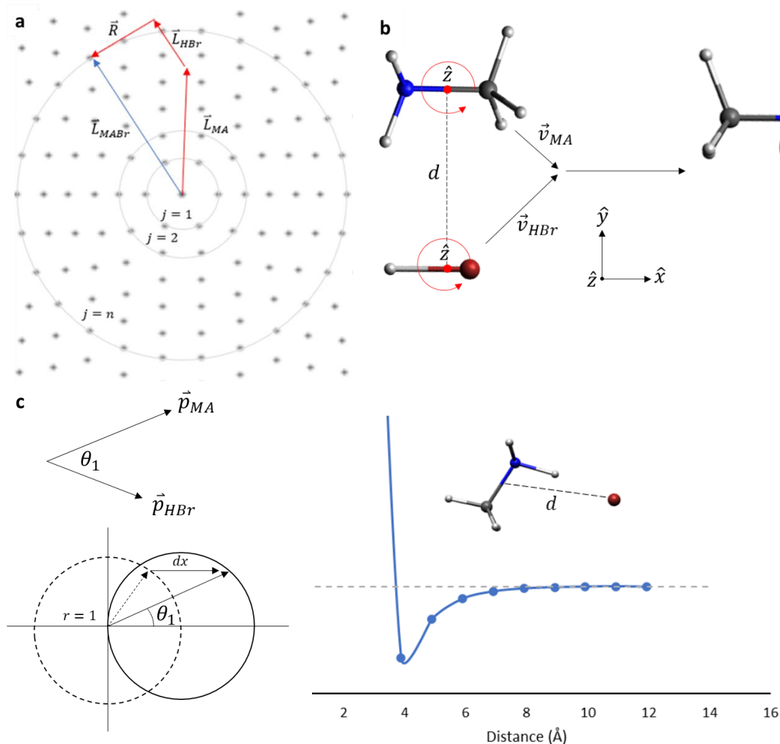
Figure 5-7: (a) Illustration of the difficulty in having all three initial angular momentum vectors add successfully to obtain a rotational eigenstate in the adduct. (b) Illustration of a simulated collision whereby the precursors' and adduct's angular momenta are aligned along the same axis, and the precursors “react” at a fixed distance, d , after colliding in the \overline{xy} plane. (c) Schematic of how the random collision angle was selected along with Equations (5-1), (5-11), and (5-12). (d) Potential energy diagram of the separation of centers of mass of the colliding precursors. The reaction was therefore assumed to occur at 4, 5, and 6 Å for 3 separate simulation series.
