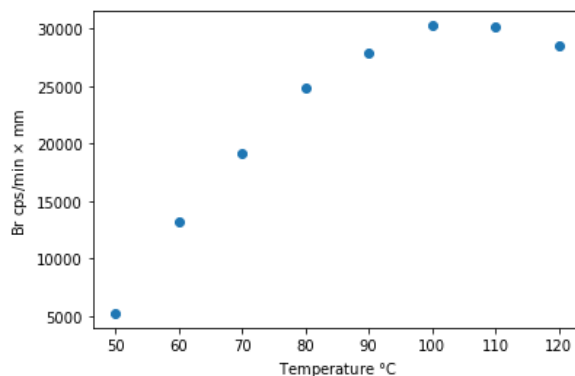
Figure 4-23: Integral of the Br EDS intensity data in Figure 4-22. The data clearly show a plateauing beginning around 100 °C and a possible reduction in growth rate at 120 °C.
