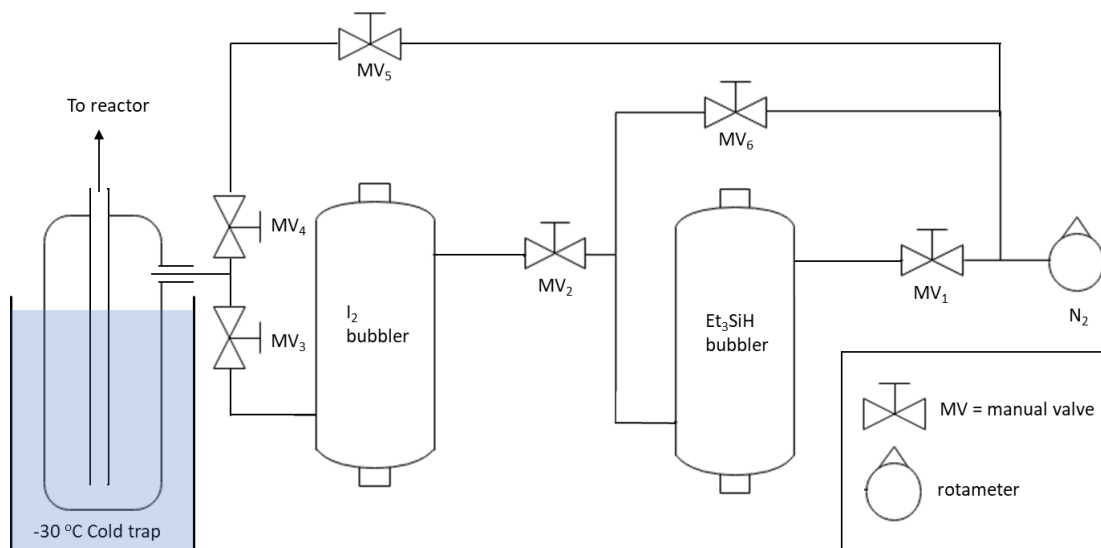
Figure 2-14: In situ HI generation schematic
