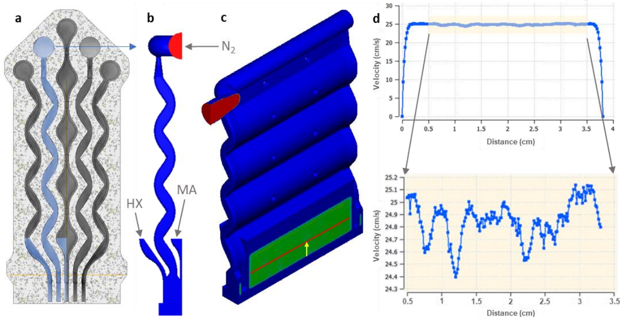
Figure 3-15: (a) The half-section view of the inlet manifold shows the baffle-like channels. The blue region was simulated to measure the uniformity of the gas flowing across the N 2 channel in the deposition zone. A significant reduction in CPU and memory requirements was obtained by not including the rest of the reactor geometry in the simulation. (b) The side profile of the simulation shows the entrance of N 2 into the inlet manifold as red (indicating a high flow rate) and blue along the walls (indicating zero flow). (c) An isometric view of (b) shows the channel near the deposition zone. The green color shows the uniformity of the flow velocity, and (d) shows a slice of the channel (red line in (c)) to highlight the magnitude. The lower velocity plot highlights the velocity variability and uncertainty in the simulation.
