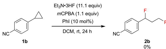
Scheme S1.2 Et 3 N•3HF as a fluoride source.
