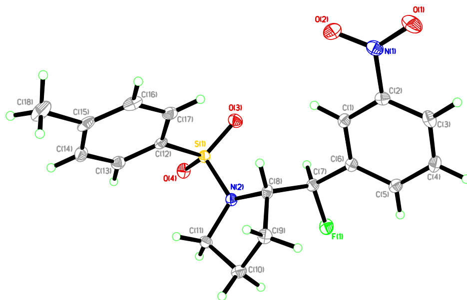
Figure S2.10 Perspective views showing 50% probability displacement.
