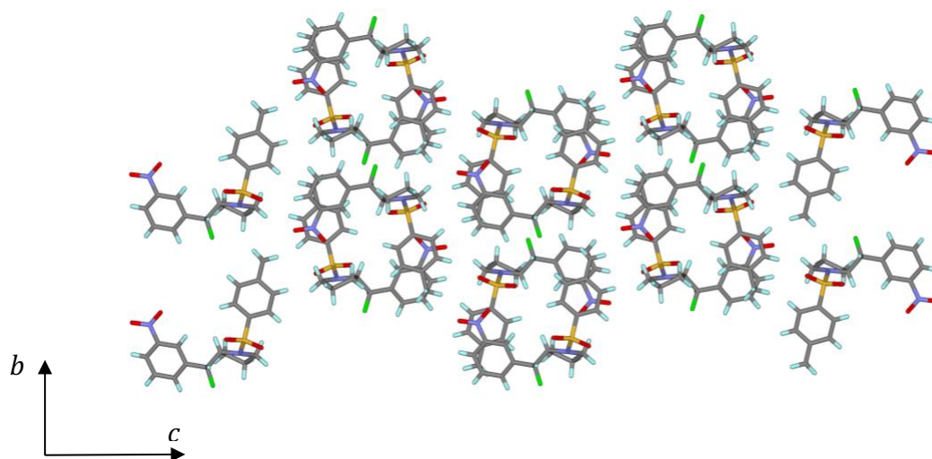
Figure S2.11 Three-dimensional supramolecular architecture viewed along the a -axis direction.
