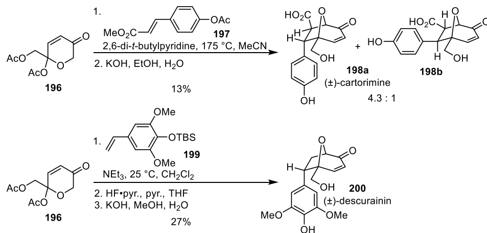
Scheme 1.33. Snider's total syntheses of cartormine and descurnin.
