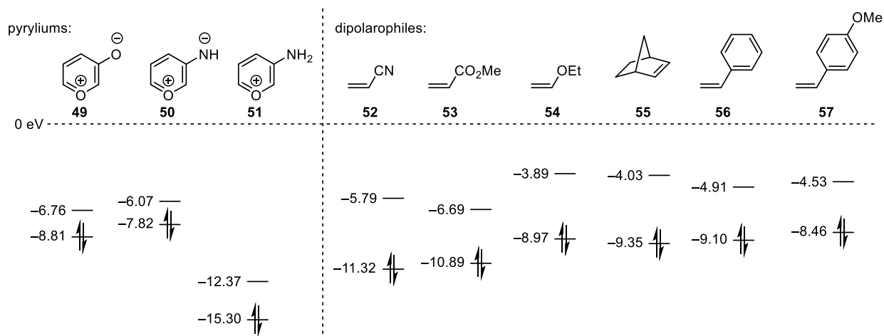
Figure 2.2. Predicted HOMO–LUMO interactions (Dr. Noah Z. Burns). Energies in terms of eV.
