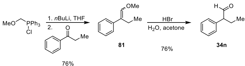
Scheme 5.33. Synthesis of substrate 34n .
