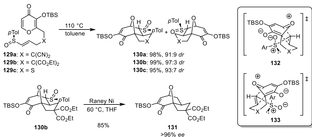
Scheme 1.19. Sulfinyl-directed [5 + 2] oxidopyrylium cycloadditions.
