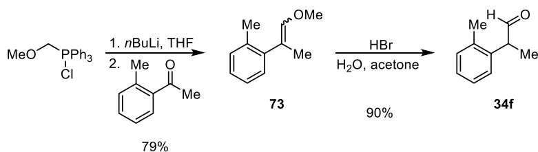
Scheme 5.25. Synthesis of substrate 34f .
