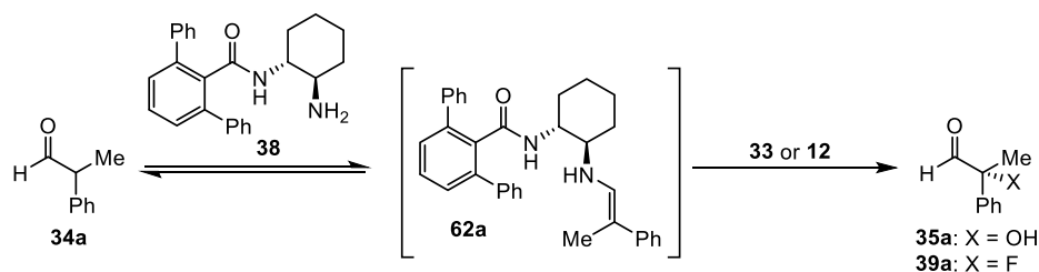
Scheme 5.16. Formation of proposed intermediate 62a .
