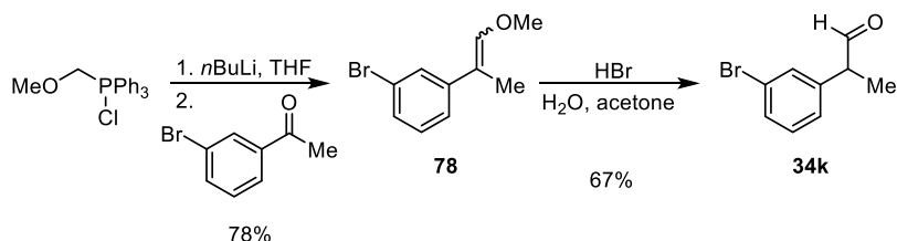
Scheme 5.30. Synthesis of substrate 34k .
