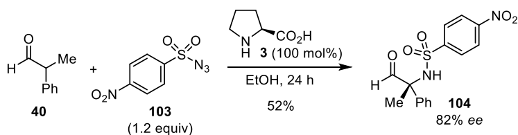
Scheme 4.9. An \alpha -amination with a sulfonyl azide.
