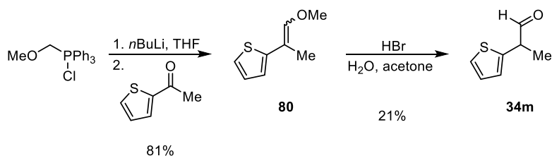
Scheme 5.32. Synthesis of substrate 34m .
