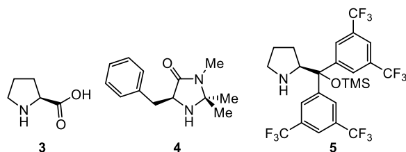
Figure 4.1. Common secondary amine catalysts.
