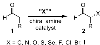
Scheme 5.1. Amine-catalyzed \alpha -functionalizations of linear aldehydes.
