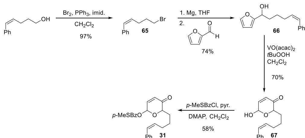
Scheme 2.12. Synthesis of substrate 31 .
