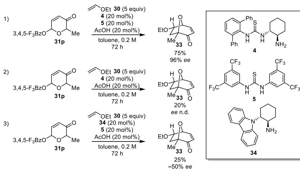
Scheme 3.8. Comparison of catalytic conditions from Chapter 2.
