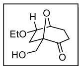
(1 R ,5 S ,6 S )-6-ethoxy-1-(hydroxymethyl)-8-oxabicyclo[3.2.1]octan-2-one (76):
