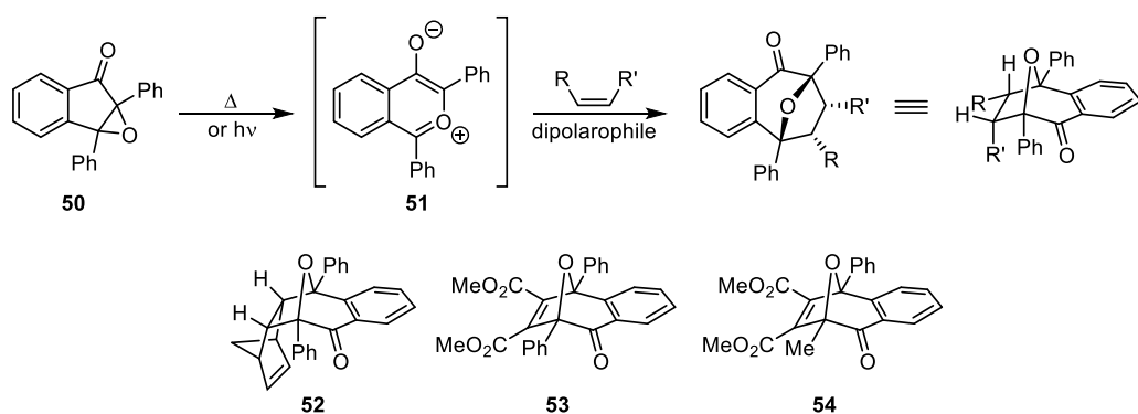
Scheme 1.8. The [5 + 2] cycloaddition of benzoperilylums derived from epoxyindanones.
