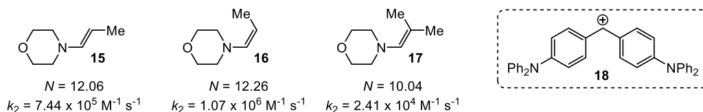
Figure 4.2. Nucleophilicity parameters of representative enamines.
