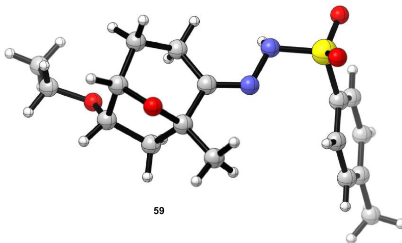
Figure 3.6. X-ray crystal structure of 59 .
