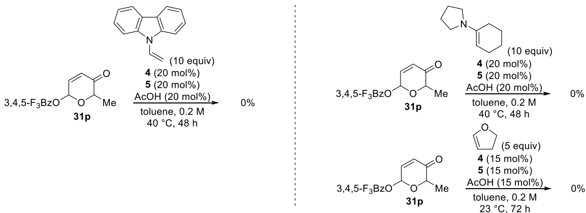
Scheme 3.21 (continued).
