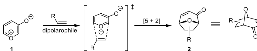
Scheme 1.1. The [5 + 2] oxidopyrylium cycloaddition.
