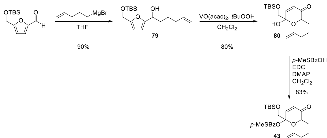
Scheme 2.18. Synthesis of substrate 43 .
