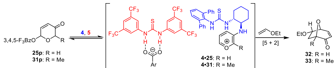
Scheme 3.10. Formation of the intermediate aminopyrylium ion pair.
