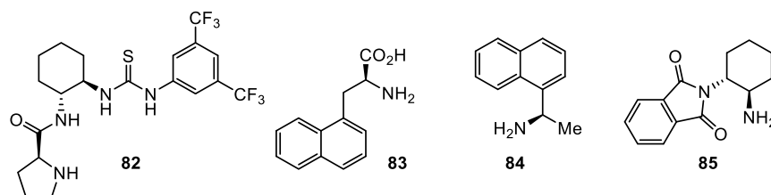
Figure 4.3. Xu and Wang's \alpha -amination catalysts.
