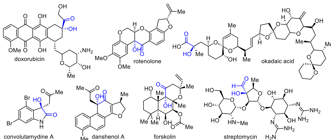
Figure 5.1. Tetrasubstituted \alpha -hydroxycarbonyls in selected natural products.
