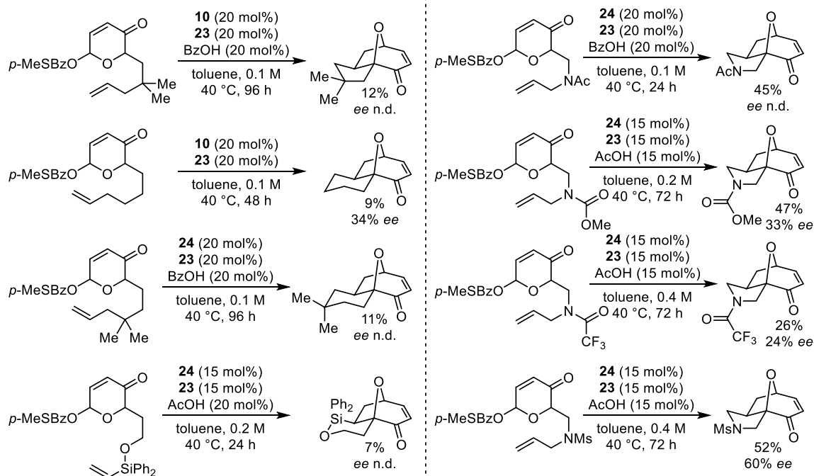
Scheme 2.19 (continued).
