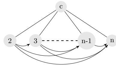
Figure 2: Cone of a Directed Acyclic Graph
