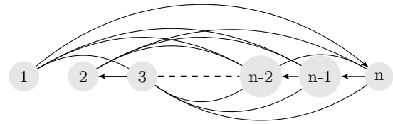
Figure 3: Counterexample to the extension lemma.
